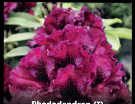
Rhododendron (T) 'Midnight Beauty'®
