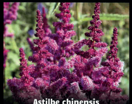
Astilbe chinensis 'Vision in Red'
